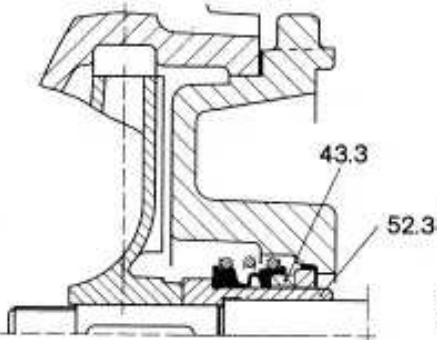
Unbalanced, uncooled single mechanical seal
