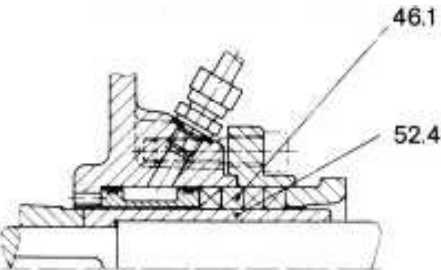
Soft packed stuffing box designed for intensive cooling
