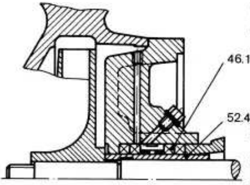
Soft packed stuffing box with sealing fluid supplied from an outside source and flushing
